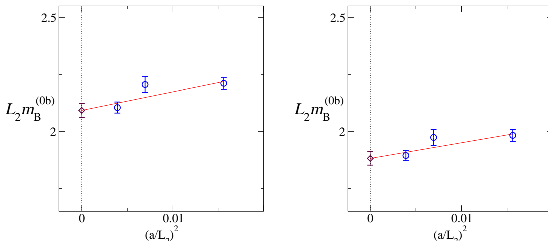
Figure 6: Lattice spacing dependence of L_2m_B^{(0b)} , details as in Fig. 5.
