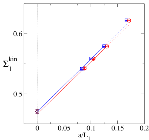
Figure 4: Continuum extrapolation of \Sigma_1^{\text{kin}} for \theta_1 = 1/2, \theta_2 = 1 .
