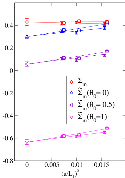
Figure 3: Continuum extrapolation of \Sigma_m and \widetilde{\Sigma}_m .
