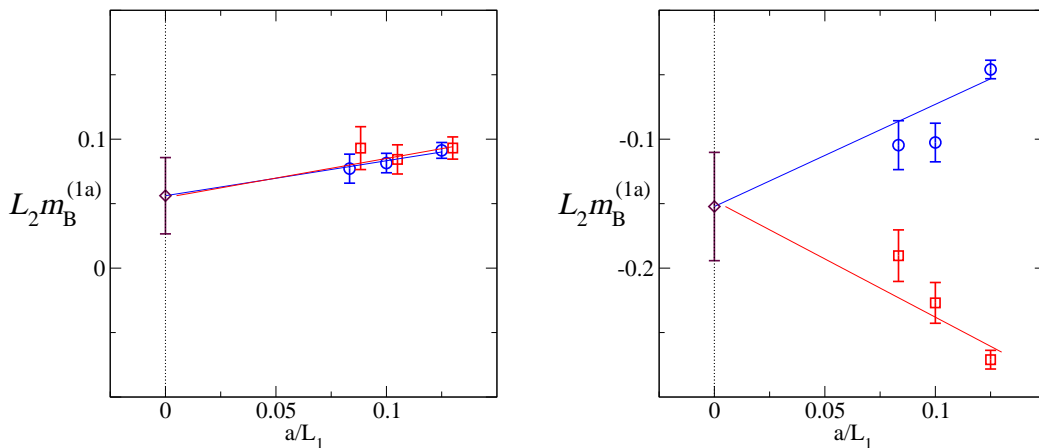
Figure 5: Lattice spacing dependence of L_2m_B^{(1a)} for M_b = M_b^{(0)} . On the left we show m_B^{(1a)} as introduced in section 4, with \theta_1 = 1/2 , \theta_2 = 1 . We insert \Phi_1 in the continuum limit, such that the lattice spacing dependence is just due to \Sigma_2^{\text{kin}} . On the right the corresponding quantity is shown for the alternative strategy of appendix C, again with continuum values for \tilde{\Phi}_i . There we set \theta_0 = 1/2 , \theta_1 = 1/2 , \theta_2 = 1 .
